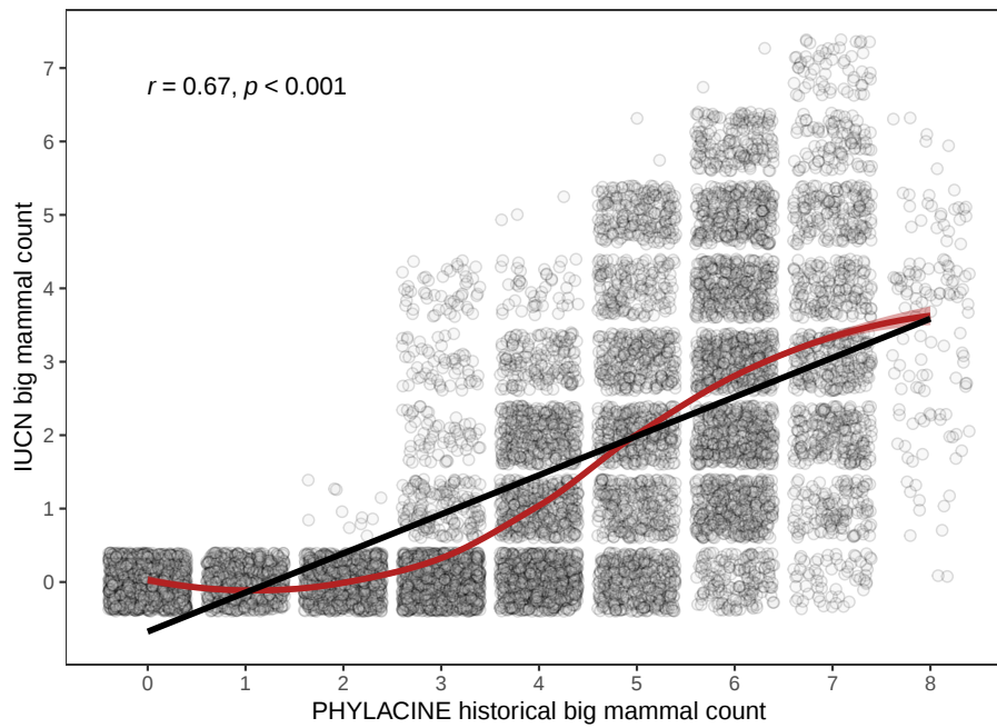
Figure A11: Correlation between IUCN and PHYLACINE large mammal presence.
