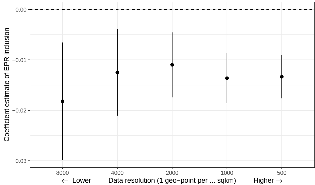
Figure A6: Robustness test: different data resolutions
