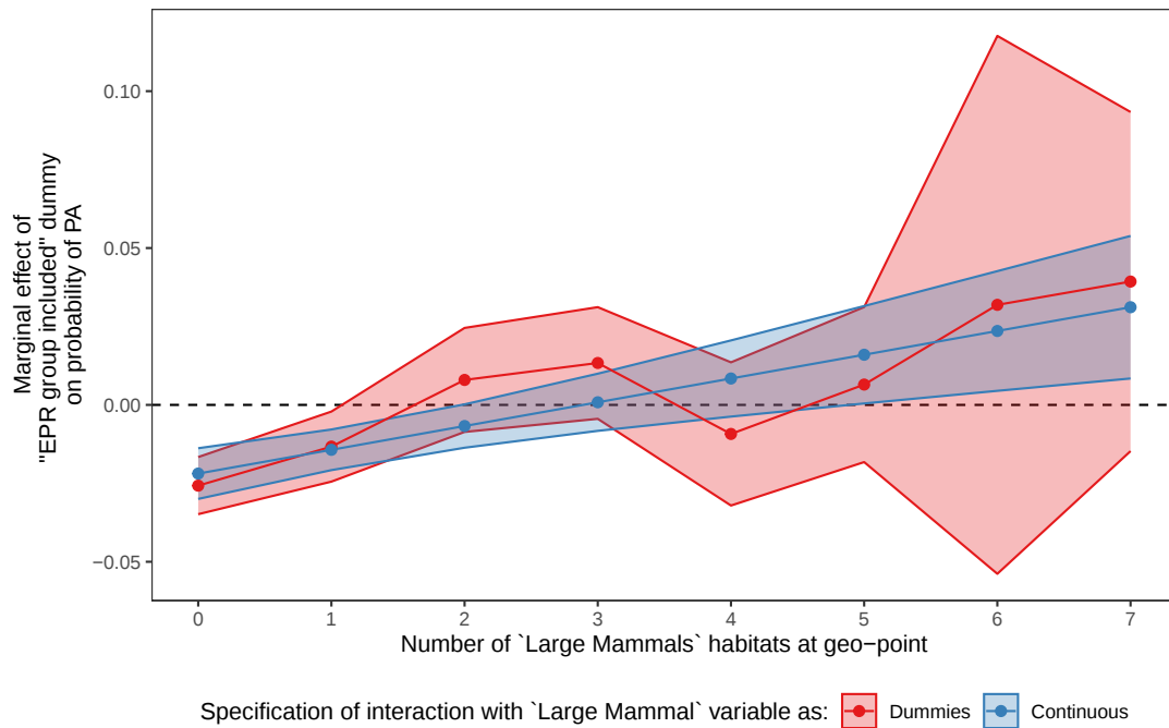
Figure 6: Marginal effects for EPR inclusion at different levels of large mammal presence
