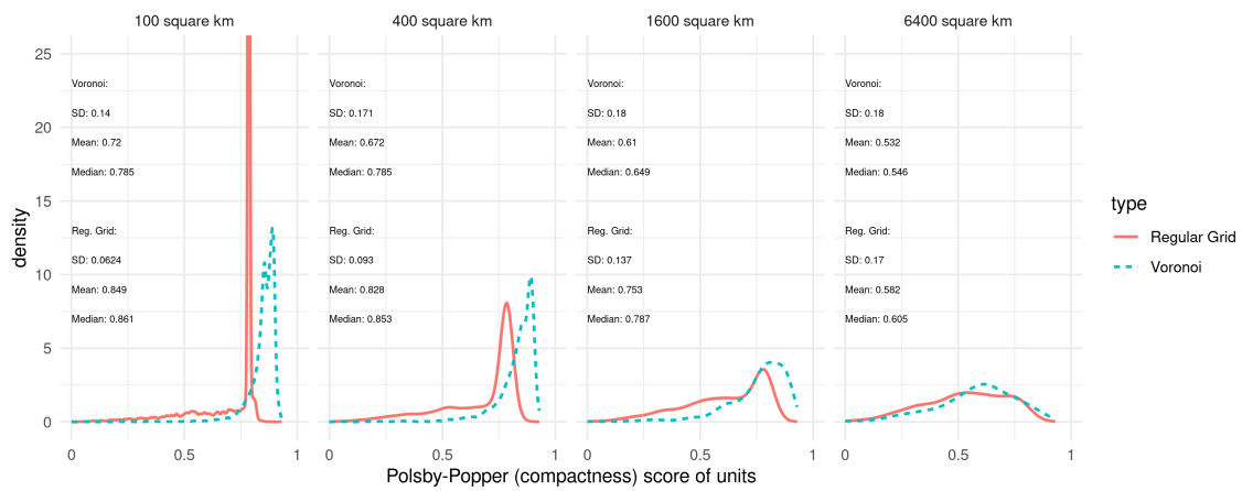
Figure A14: Compactness of Voronoi and regular grid cells for varying target sizes.
